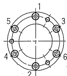
Fig. 3 Tightening sequence for bolts
